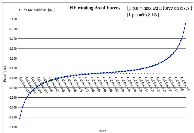
Distribution of axial forces on each HV disc [p.u.] at first peak current
