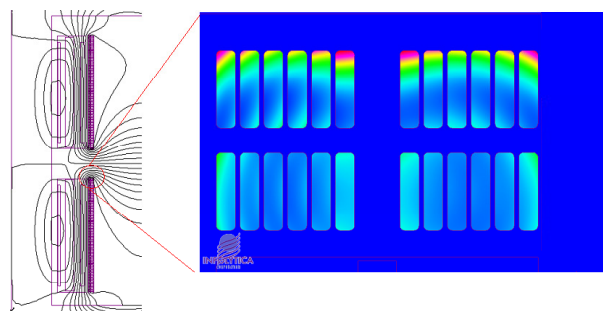
5 th , 7 th harmonic leakage flux with loss density of the affected double disks
